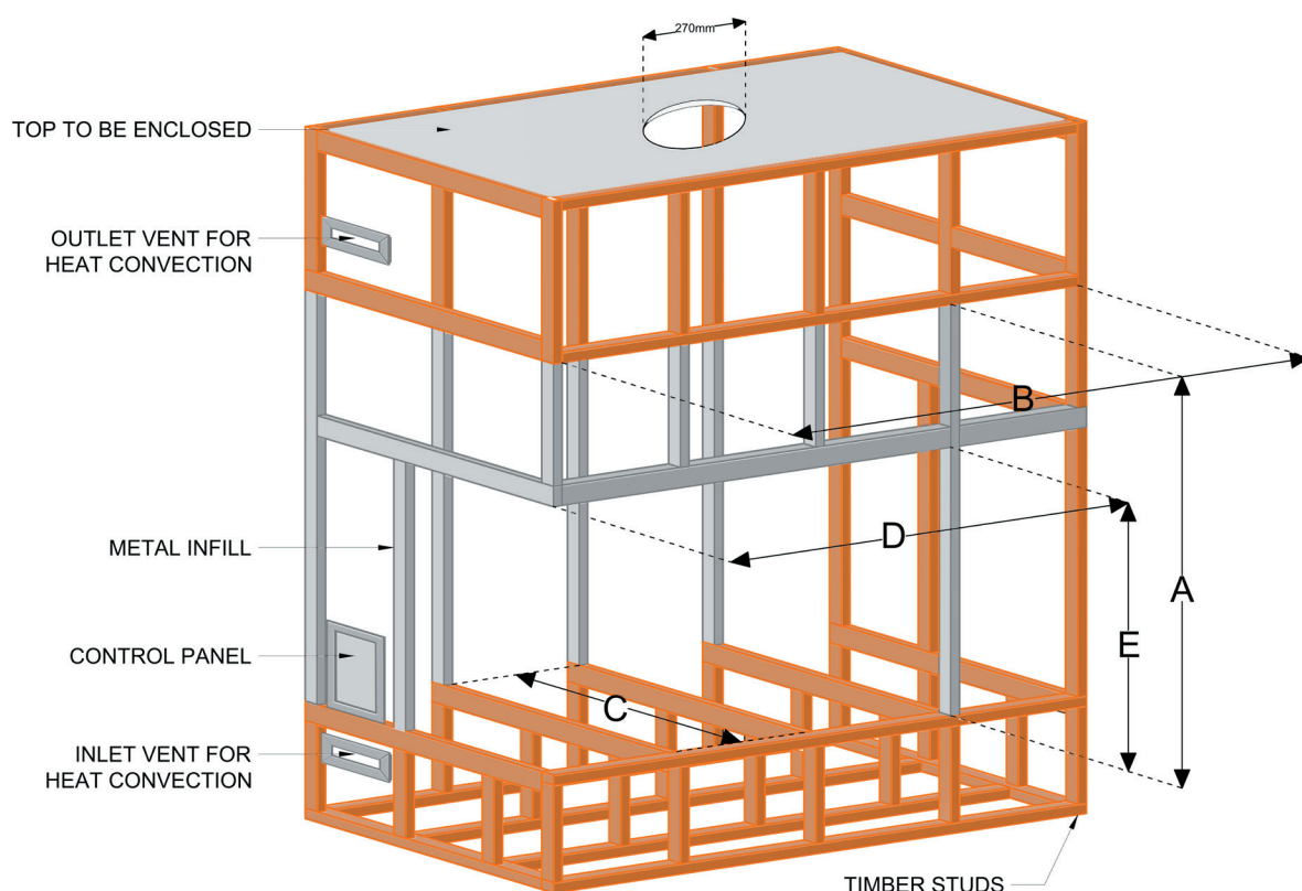
Figure 1.8 (Timber framing)
